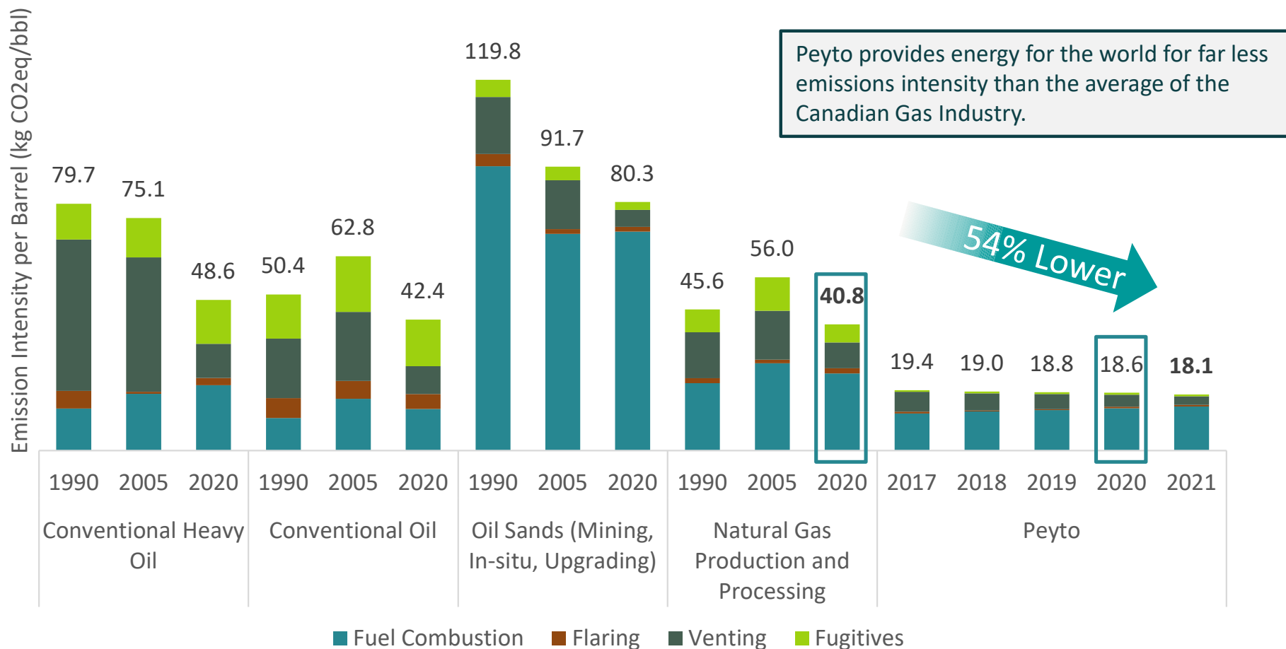
Emissions Intensity by Source Type for Canadian Oil and Gas (1990, 2005, 2020)
