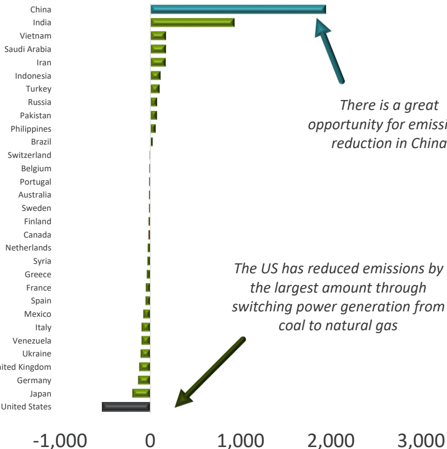
Absolute Change in CO2 Emissions from Fossil Fuels (2011-2021) (million tonnes of CO2)
